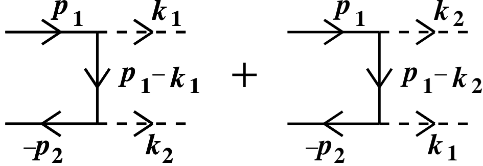
Figure 6: Diagrams for e^+e^- \rightarrow \varphi\varphi , corresponding to eq. (497).
