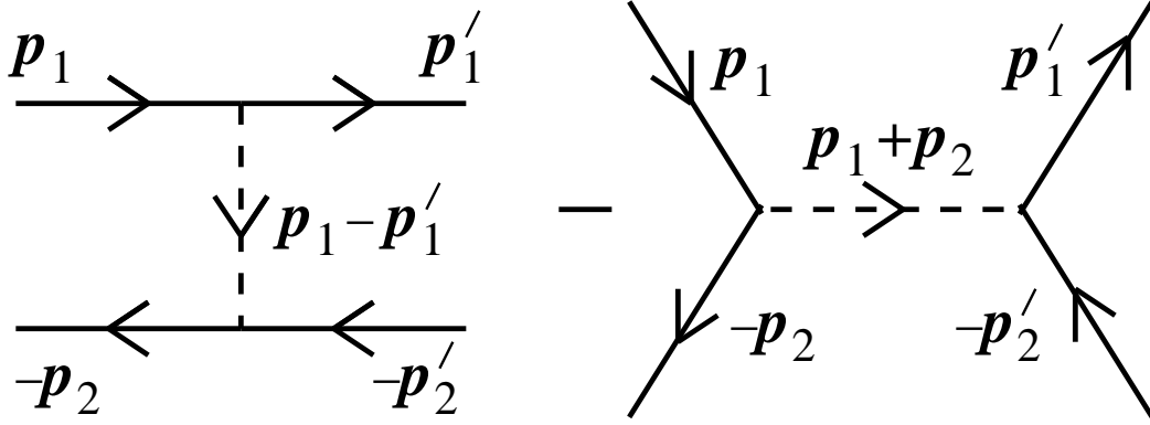
Figure 8: Diagrams for e^+e^- \rightarrow e^+e^- , corresponding to eq. (499).
