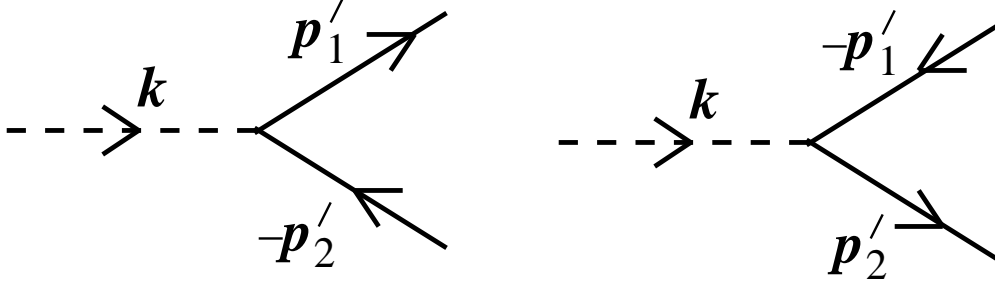
Figure 10: Two equivalent diagrams for \varphi \rightarrow \nu\nu , corresponding to eqs. (569) and (570), respectively.
