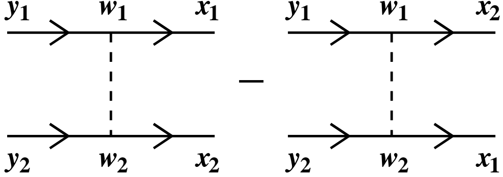
Figure 3: Diagrams corresponding to eq. (484).
