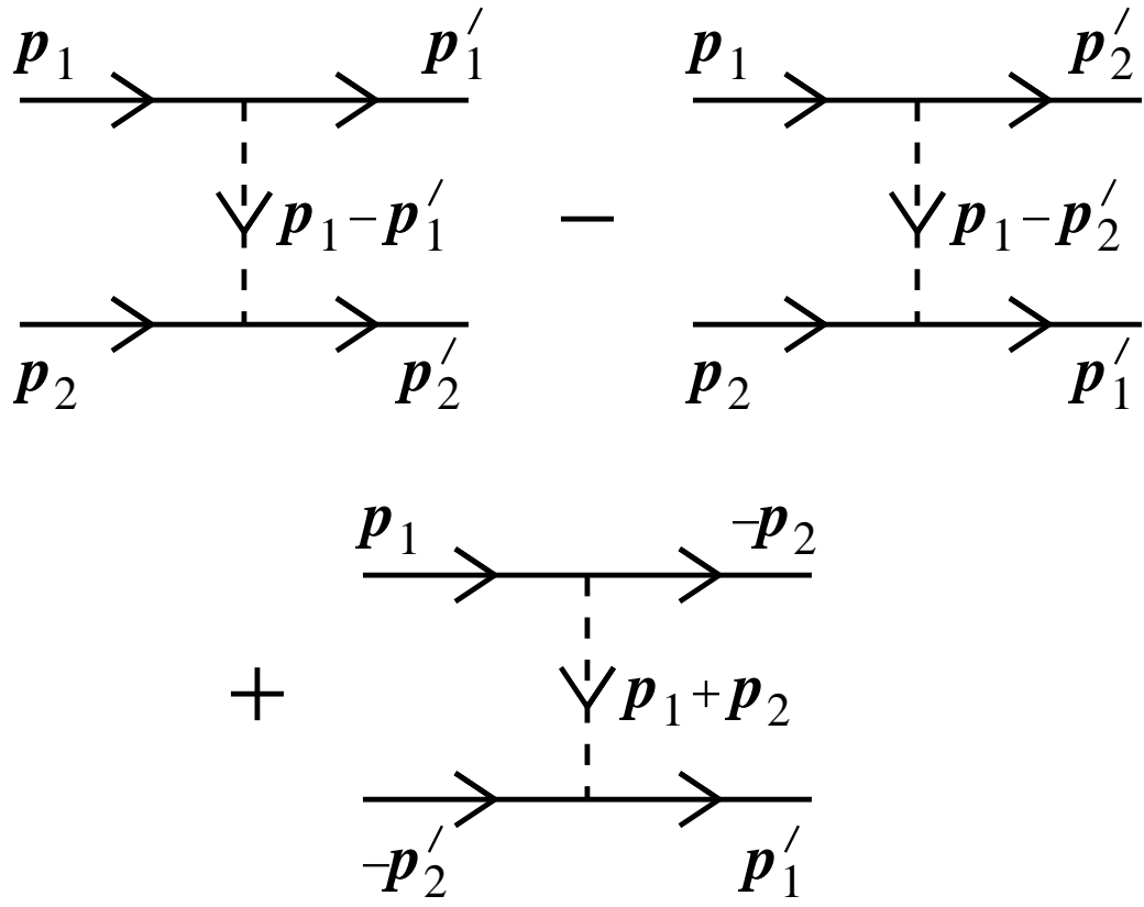
Figure 11: Diagrams for \nu\nu \rightarrow \nu\nu , corresponding to eq. (572).
