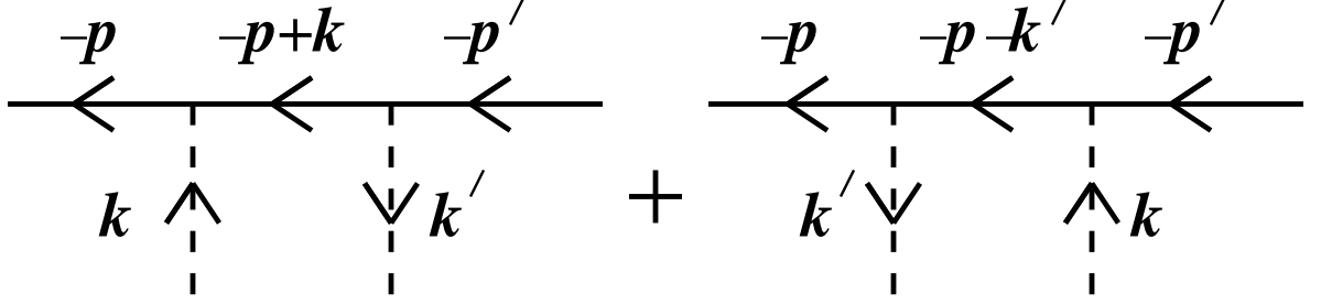
Figure 5: Diagrams for e^+\varphi \rightarrow e^+\varphi , corresponding to eq. (496).
