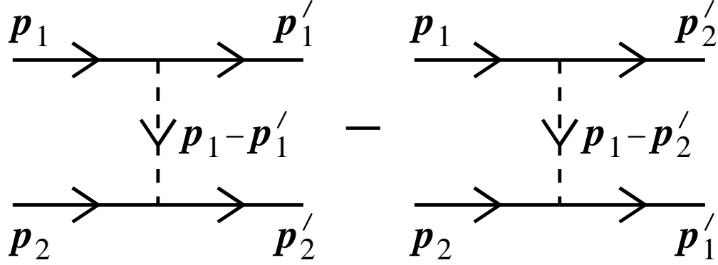
Figure 7: Diagrams for e^-e^- \rightarrow e^-e^- , corresponding to eq. (498).
