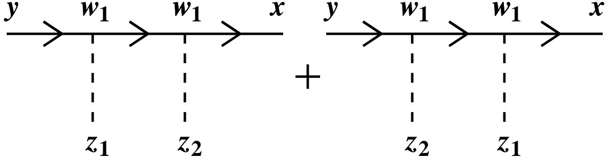
Figure 2: Diagrams corresponding to eq. (482).
